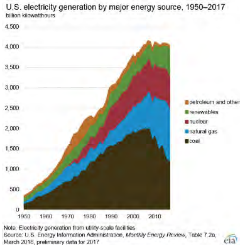
Figure 5.2.1: Types of fuels used in electricity production
